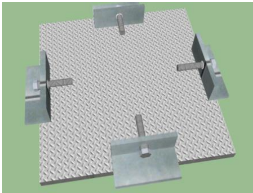
Fig. 1 Assembly for testing
