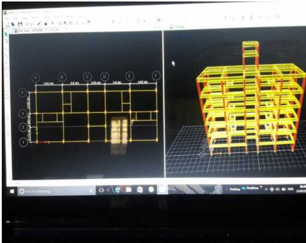
Structural design in ETABS
